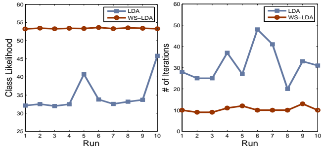
Figure 2: Comparisons between WS-LDA and LDA on (a) Overall Class Likelihood on Testing Set, (b) Convergence Speed on Training Set
