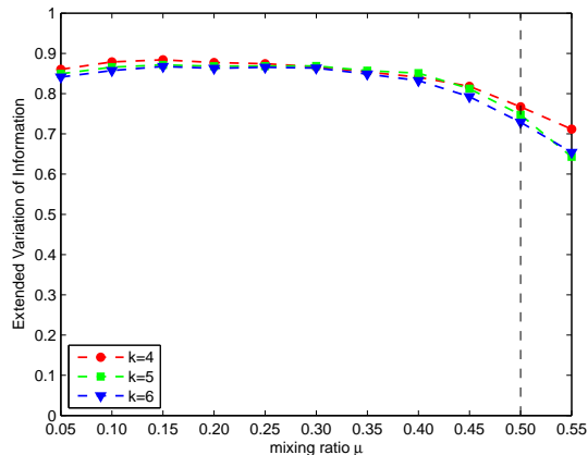
FIG. 4: Test of our method on the benchmark networks. The parameter k in the legend corresponds to the parameter k in our method. The threshold \mu = 0.5 (dashed vertical line in the figure) marks the border beyond which communities are no longer defined in the strong sense [28], i.e., such that each node has more neighbors in its own community than in the others. Each point corresponds to an average over 100 graph realization.
