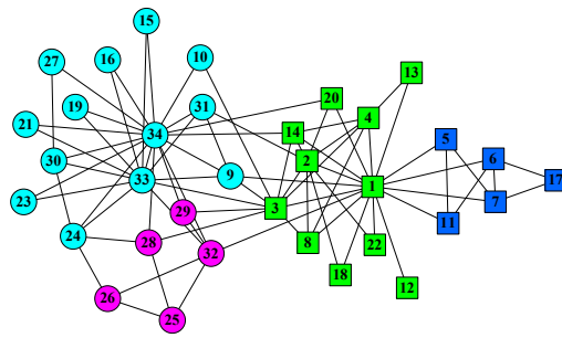
FIG. 5: The network of the karate club studied by Zachary [29]. The real social fission of this network is represented by two different shapes, circle and square. The different colors show the partition obtained by our method with the parameter k = 4 .
