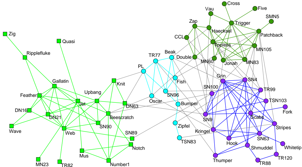
FIG. 6: The community structure identified by our method from the network of the bottlenose dolphins of Doubtful Sound. The primary split of the network is represented by different shapes, square and circle. The different colors show the partition obtained by our method with the parameter k = 4 .
