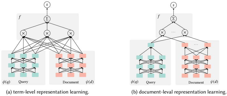
Fig. 3. Different dense retrieval models for the first-stage retrieval.
