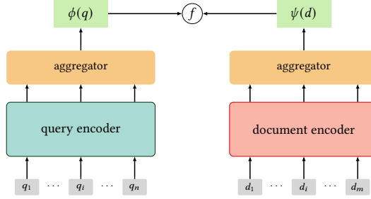
Fig. 2. Dual-encoder architecture of dense retrieval methods.
