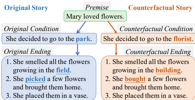
Figure 1: An example of an original story and counterfactual story pair. Black words in the two endings are background content, colored words are causal content.
